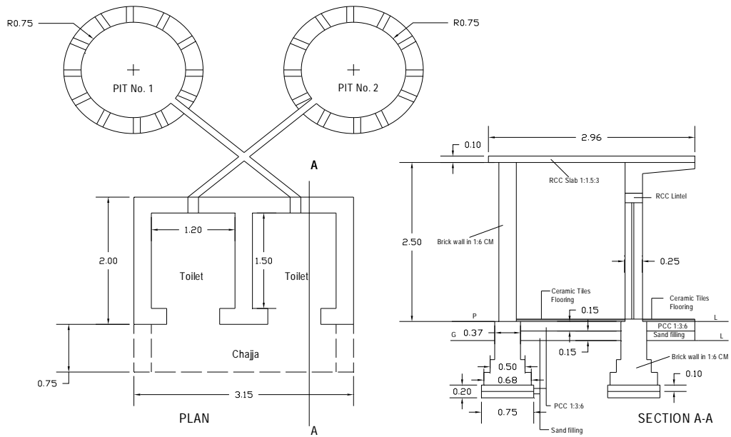
Construction Twin Pit Toilet at Bhadrasai Mines Roida under CSR Scheme
