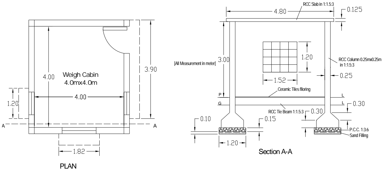
Construction of a weigh cabin (4m x 4m) inner size for installation of inmotion weighbridge at Thakurani Siding.
